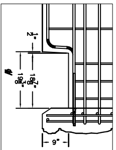
DETAIL OF NOTCH FROM SECTION A-A SCALE: 3/4"=1'-0"
