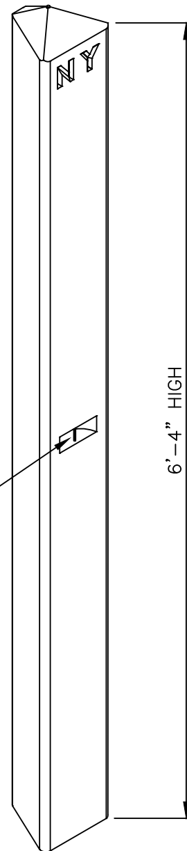
H-TYPE RIGHT OF WAY MARKER
