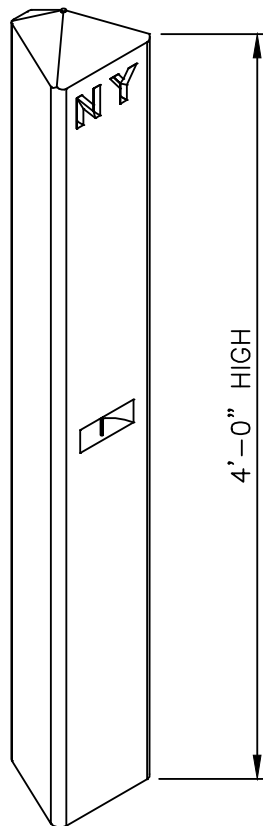
L-TYPE RIGHT OF WAY MARKER
