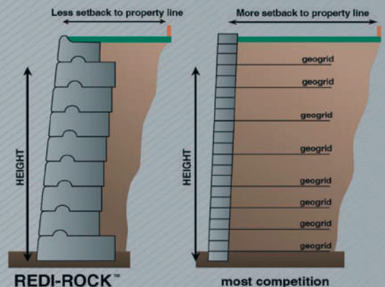
Redi-Rock blocks harness the power of gravity. Smaller block systems require time-consuming and costly reinforcement to reach the same heights.
