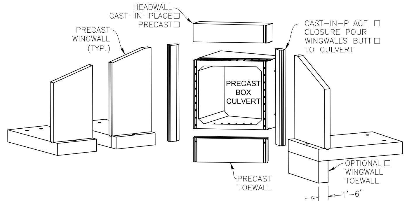
EXPLODED VIEW
