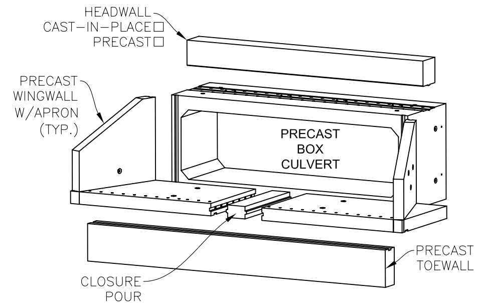
EXPLODED VIEW
