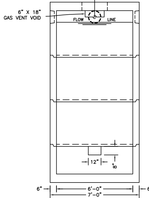
SECTION B-B
