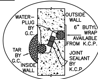
WATERTIGHT JOINT DETAIL SCALE: N/A
