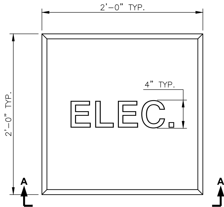
PLAN VIEW ELECTRIC MARKER
