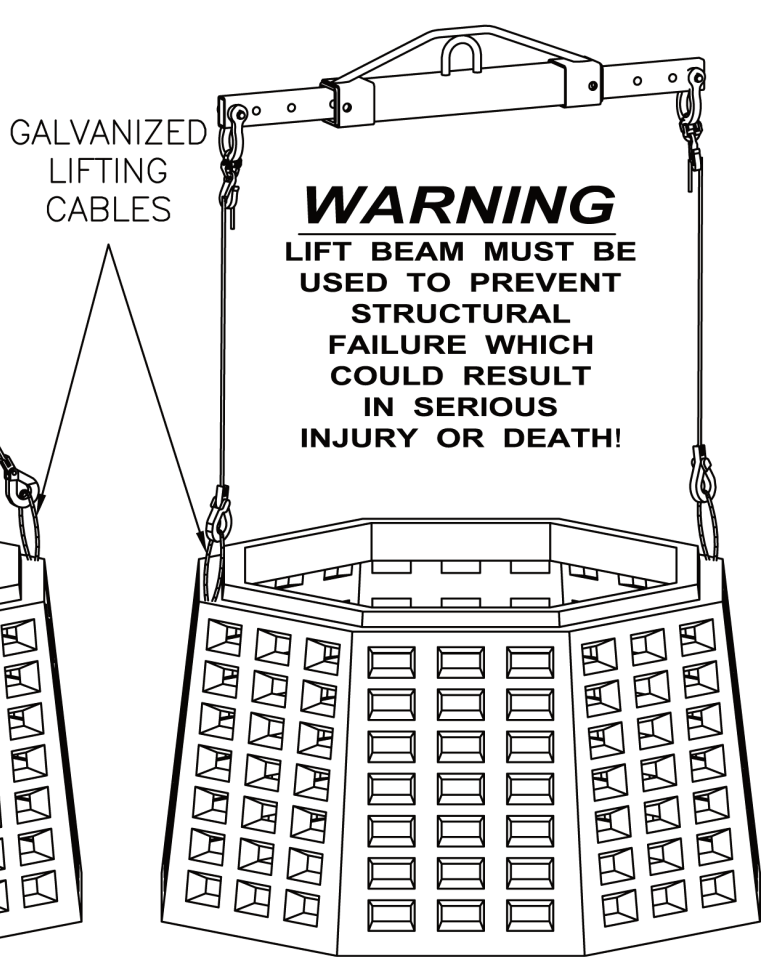
TYPES B & R (NO ROOF SLAB)
