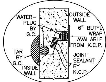
WATERTIGHT JOINT DETAIL SCALE: N/A
